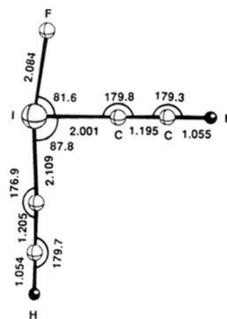
12, IF(CCH) 2 ( C_s , 1A' )
