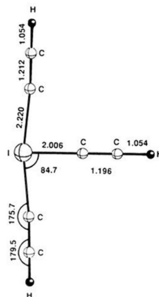
14, I(CCH) 3 ( C_{2v} , 1A_1 )
