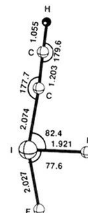
11, IF 2 CCH ( C_s , 1A' )
