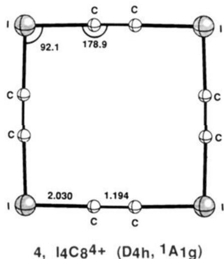
Figure 2. Calculated geometries (bond lengths in angstroms, angles in degrees) of square planar tetracation 4.
