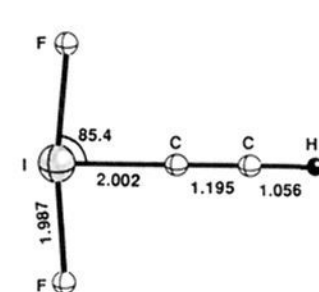
10, IF 2 CCH ( C_{2v} , 1A_1 )
