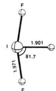
15, IF 3 ( C_{2v} , 1A_1 )
