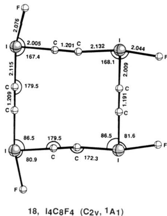
Figure 3. Calculated geometries (bond lengths in angstroms, angles in degrees) of square tetraalkynyl tetraiodonium molecules 16–19.
