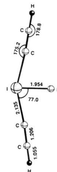
13, IF(CCH) 2 ( C_{2v} , 1A_1 )
